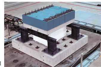
Shaking Test of NPP Concrete Wall
