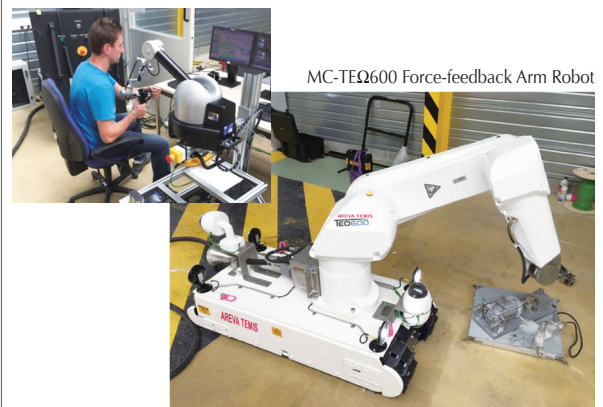
Figure 2. Remotely Controlled Robot:
