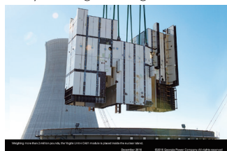
Structural Module (PWR) [Photograph provided by Georgia Power]
