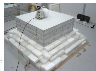
Neutron Irradiation Measurement [ 252 Cf, shielding concrete]
