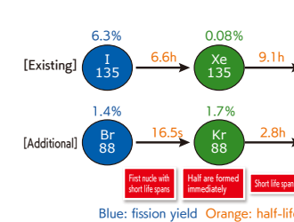
▲ Behavior of monitored nuclides
