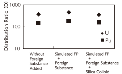
D = organic phase (water-phase total for five times back extraction) / water phase (total for two times extraction) (b) Distribution ratio of U / Pu during the presence of foreign substance
