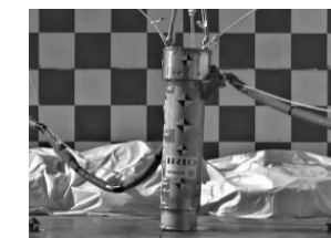
Structural test (dropped vertically)
