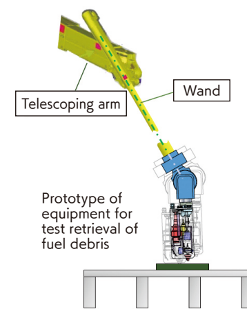
▲ Conceptual image of combination test with the arm for detailed investigation inside PCV
