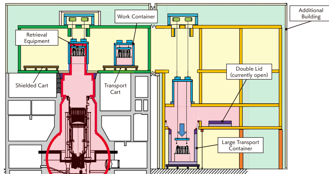
▲ Removal and transport of the entire structure
