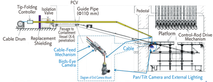
▲ Investigating the inside of Unit 2's PCV using a guide pipe (Figure 2-1)
