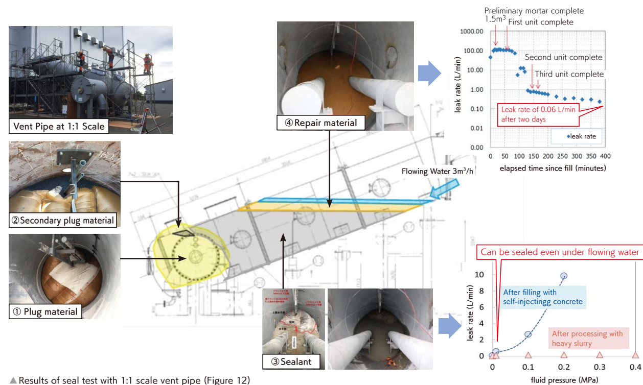
▲ Results of seal test with 1:1 scale vent pipe (Figure 12)
