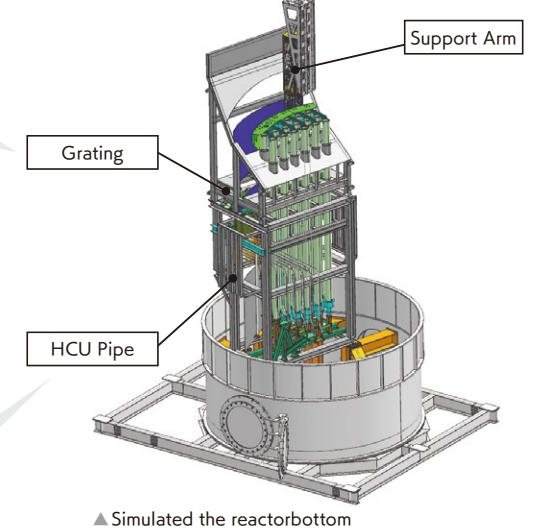
▲ Simulated the reactorbottom
