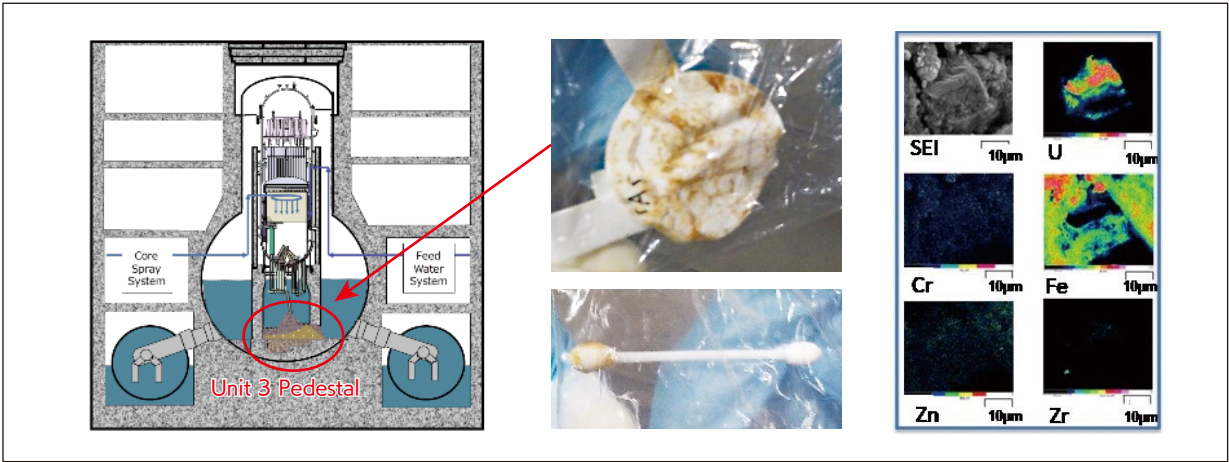
▲ Result of analyzing adhered material (Figure 19)
