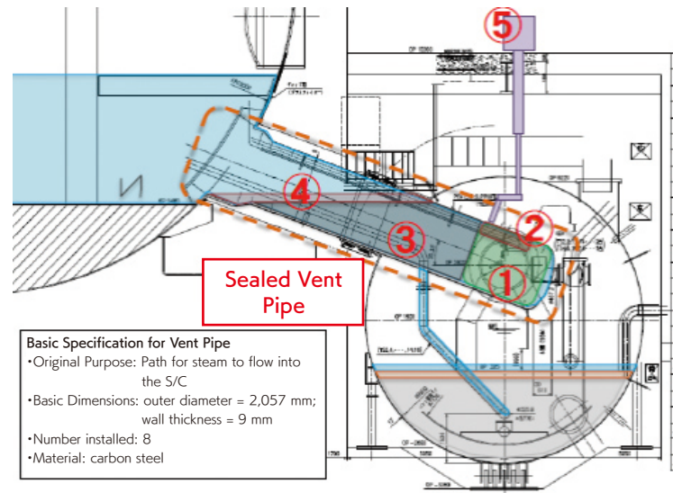
▲ Overview of the vent-pipe seal test (Figure 11)
