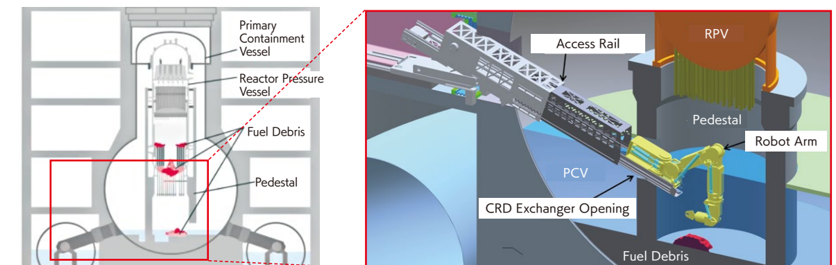
▲ Overview of side-access method
