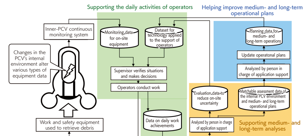
▲ Concept for on-site application of a continuous monitoring system inside the PCV (Figure 4)
