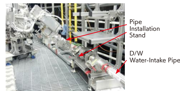
▲ Connection of D/W water-intake pipe (Figure 3)
