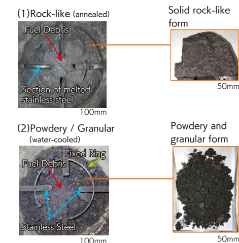
▲ Test production of melted and hardened metallic/ceramic mixture at the NNC in Kazakhstan (Figure 2)
