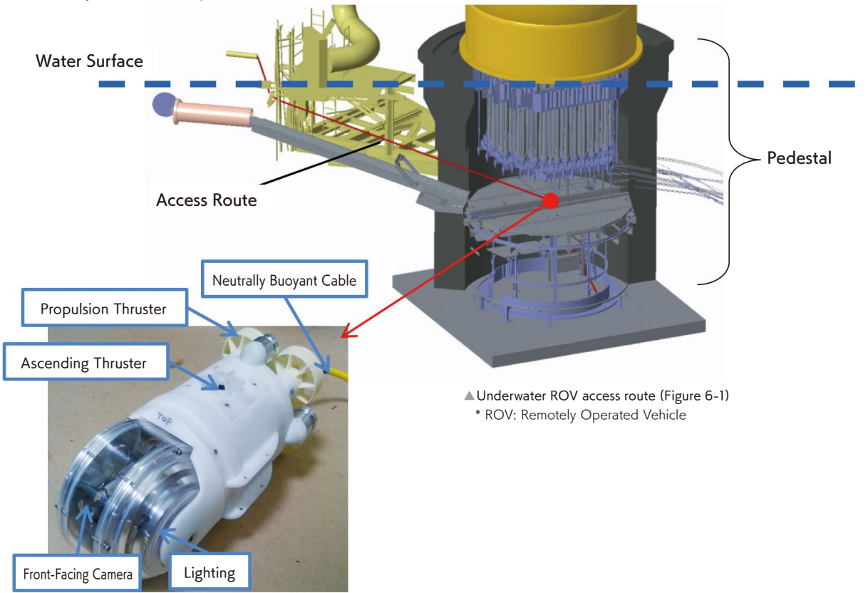
ROV Entry Point (PCV penetration)
