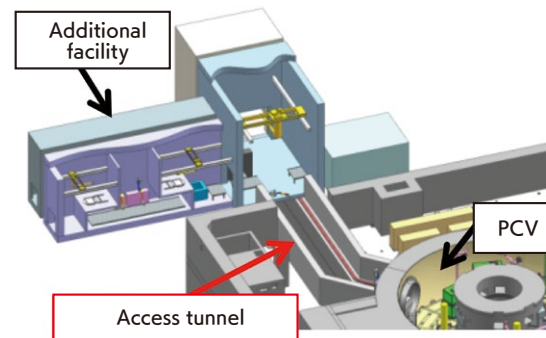
▲ Conceptual drawing of access tunnel
