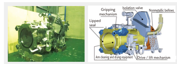
▲ Overview of the X-6 penetration connection structure (Figure 4-1)
