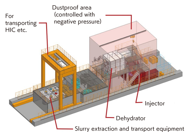
▲ The pressurized filtration process (Figure 5)
