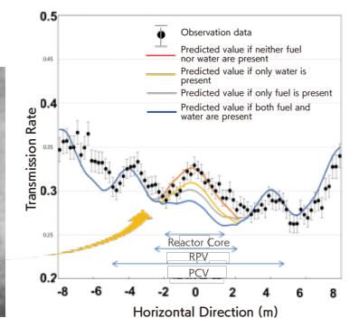
▲ Comparison of actual transmission rates and those predicted by simulations (Figure 4)
