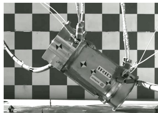
▲ Structural test (dropped at an angle) (figure 5)
