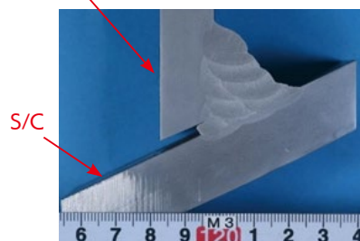
▲ Macro cross-section of weld (3 layers, 8 passes) (Figure 8)
