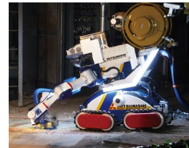
▲ Suction and blast decontamination equipment (Figure 1)
