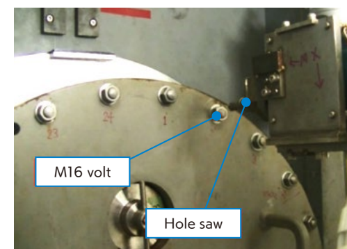
▲ Test setup of hatch release operation (Figure 5-2)
