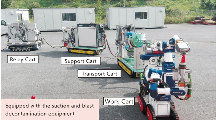
◀ Decontamination equipment for the upper floors (Figure 7)
