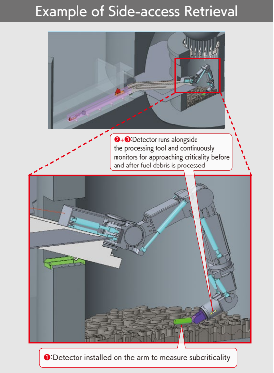
▲ Monitoring for approaching criticality when retrieving PCV fuel debris from the side
