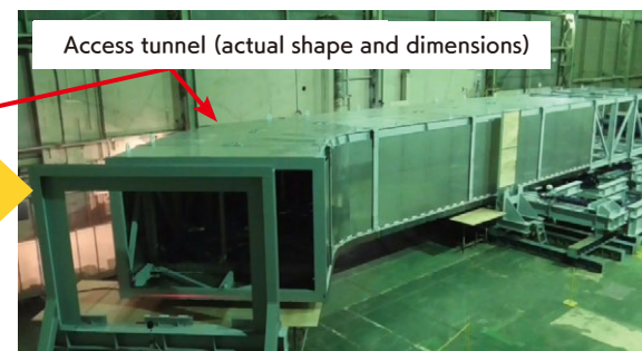
▲ Test welding the access tunnel connection
