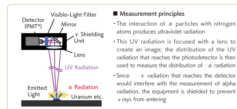
▲ Principles of the alpha camera (Figure 8)
