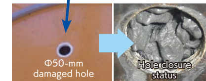
S/C damaged holes (before and after filling)
