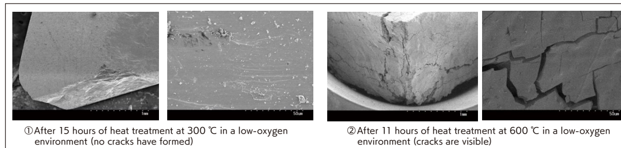
▲ Appearance of simulated fuel debris after heat treatment (Figure 12)
