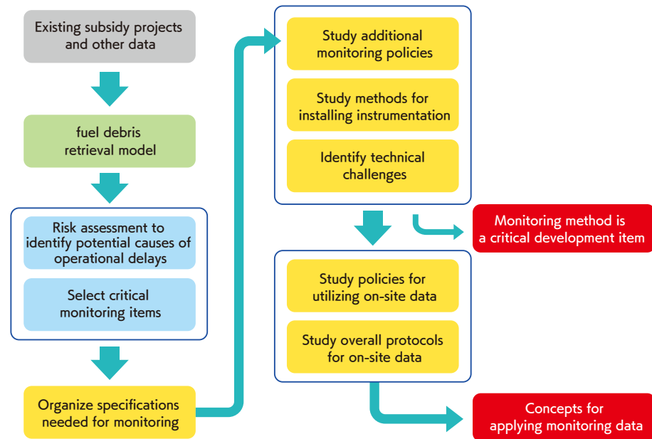
▲ Development process for a continuous monitoring system inside the PCV (Figure 1)
