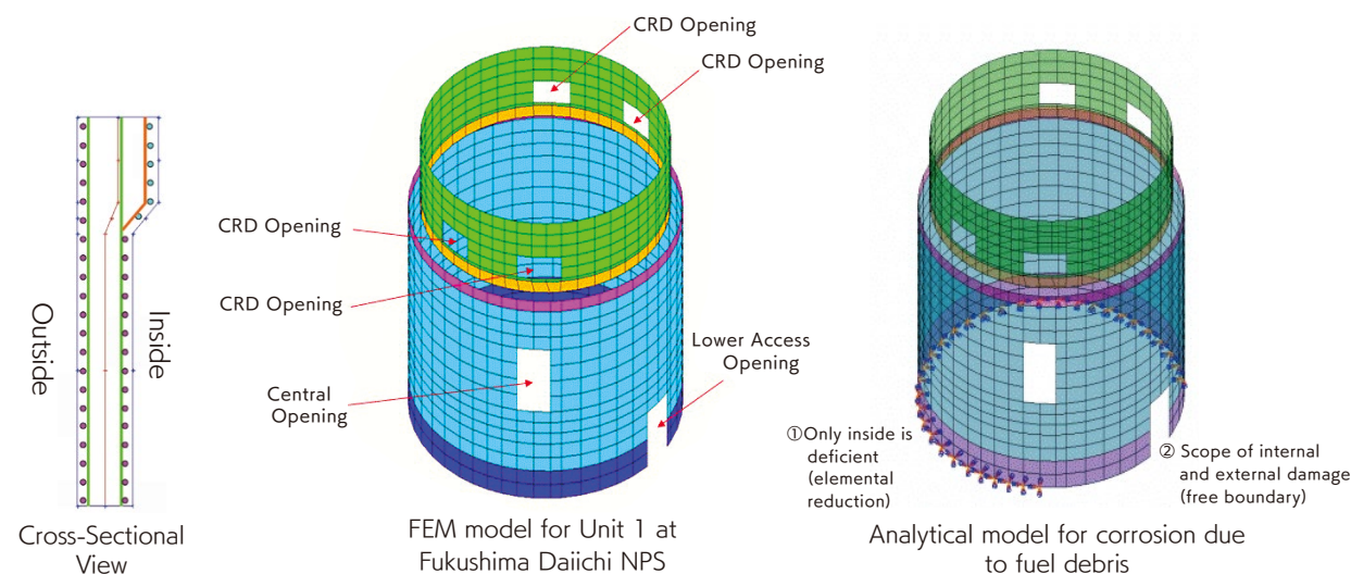
▲ Development of a method for assessing the earthquake resistance of the RPV pedestal through fuel debris corrosion (Figure 7)
