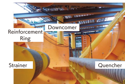
Interior of S/C (before filling)
