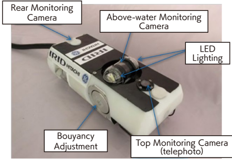
▲ The small submersible robot [IRIDOLPHIN-A2] (Figure 4-3)
