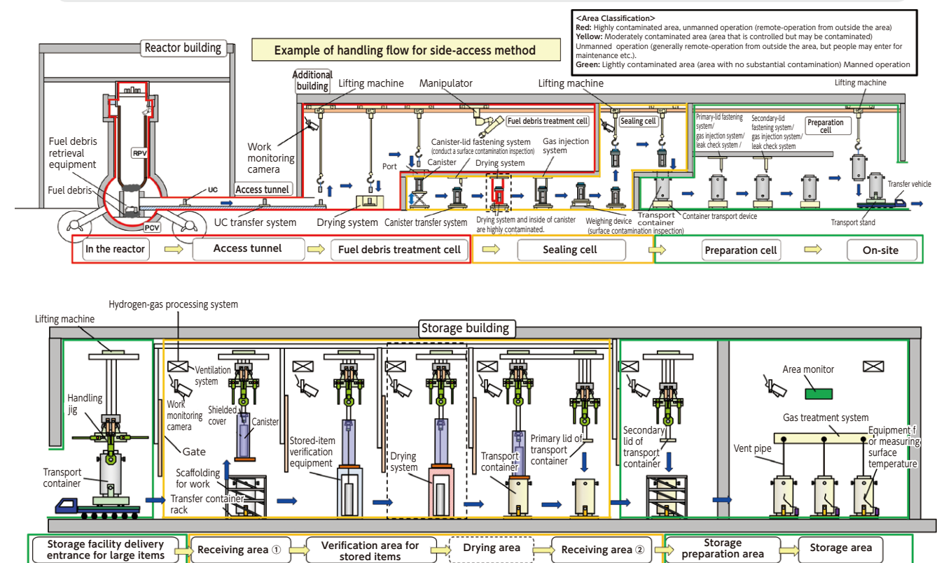
▲ Example flow based on a scenario that involves containing, transferring, and storing fuel debris (figure 1)
