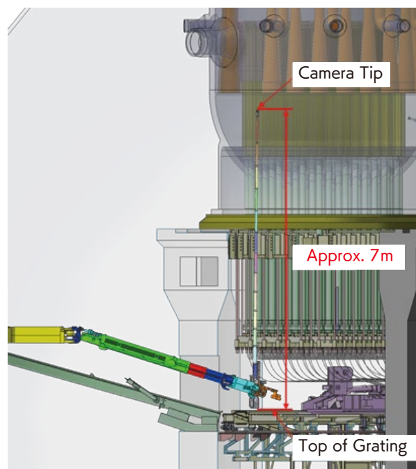
▲ Accessing Units 2 and 3 with a telescoping pipe (Figure 3)
