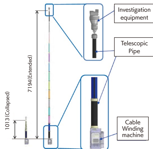
▲ Telescoping equipment (Figure 4)
