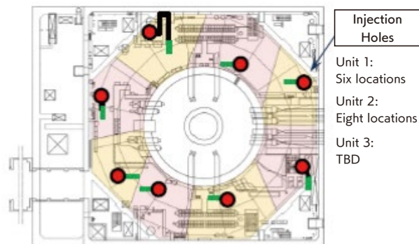
▲ Injection hole locations imagined for the reactor building's first floor (Figure 4) Maximum interval between injection holes: approximately 20 meters
