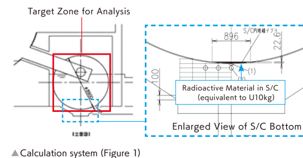
▲ Calculation system (Figure 1)
