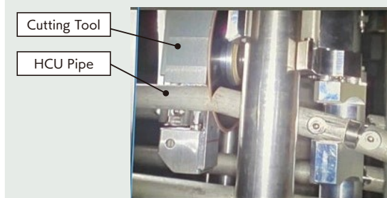
Cutting test on simulated HCU* pipe
