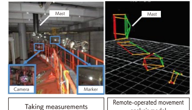
▲ Measuring movement of remote-operated equipment (photo 6)
