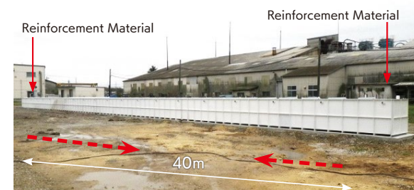
▲ Long-distance flow test (Figure 5)
