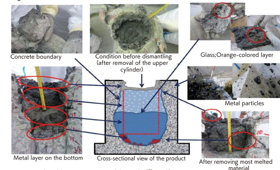
▲ Large-scale MCCI test: appearance of the results (Figure 3)
