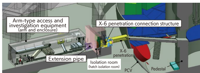
▲ Arm unit test (X-6 penetration test) (Figure 3-1)
