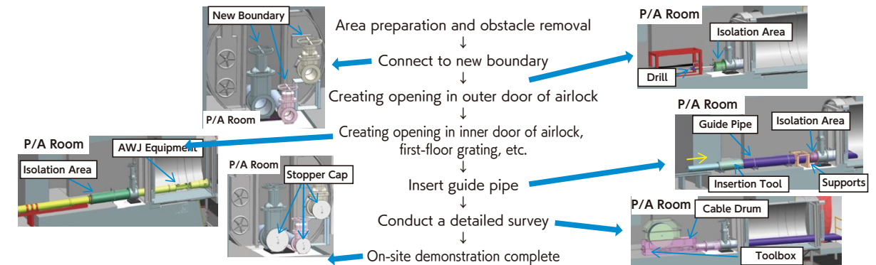
▲ Steps to create the access route (Figure 3-1)
