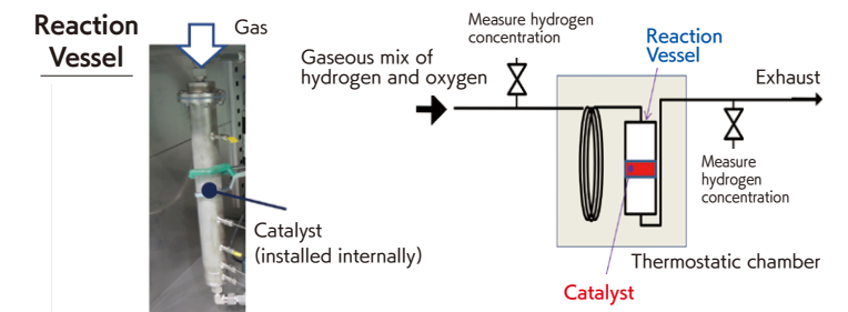
▲ Concept for testing flow reaction velocity (figure 7)
