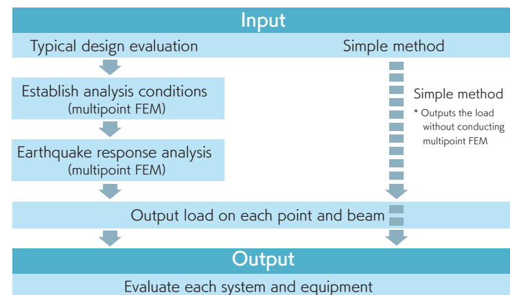
▲ Evaluation process for typical earthquake assessments and the simple method (Figure 1)
