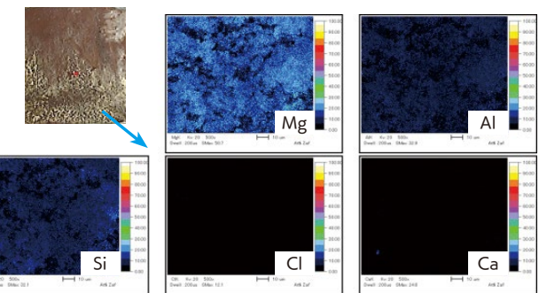
▲ Chemical analysis of white sediment on Unit 4 locknut (Figure 3)
