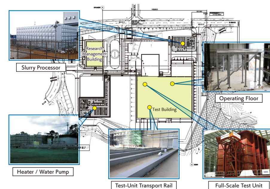
◀ Various equipment assembled for the full-scale test (Figure 1)
