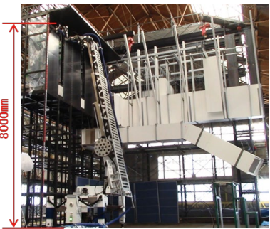
▲ Mock-up test facility (Figure 8)
