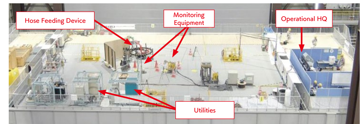
▲ Verifying workability and remote operation (Photo 9)
