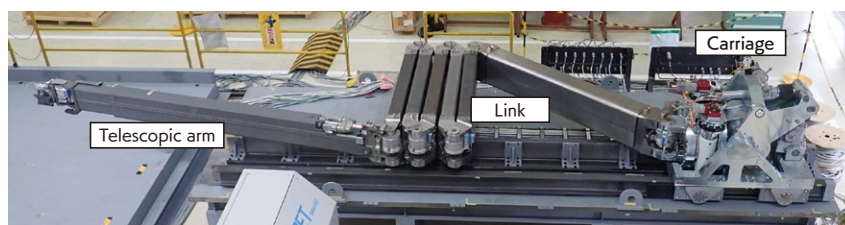
▲ Arm unit test (X-6 penetration test) (Figure 3-1)
