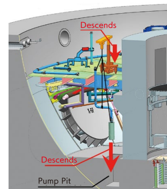
The dry-well intake line
