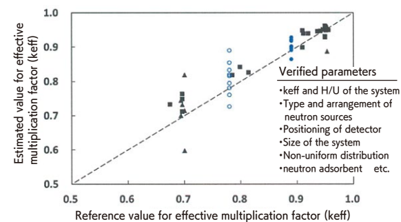
▲ Results of evaluating effective multiplication factor with the Feynman-alpha method (Figure 2)
