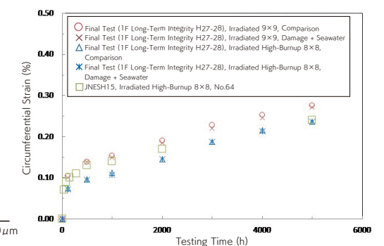
▲ Results of creep speed test (irradiated test piece, 360 °C, circumferential stress of 170 MPa, damaged, seawater adhesion, testing time of 5,000 h) (Figure 6)
