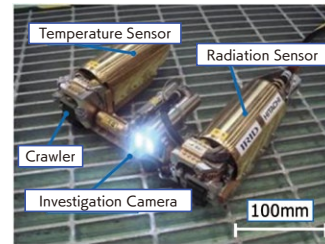
▲ PMORPH1 for investigating the first-floor pedestal exterior (Figure 1-1)
