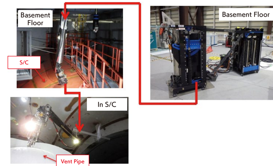
▲ Verifying the workability of remote-operated repair equipment (Photo 3)
