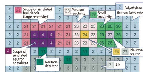
▲ Example of testing system that simulates fuel debris at KUCA (reactor core simulating the neutron adsorbent and an uneven debris distribution)
