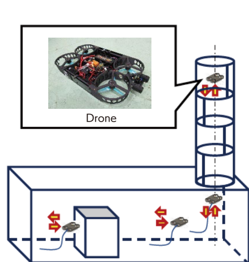
▲ Drone flight test at Unit 1 (Figure 2)
