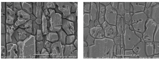
Simulated waste liquid from Rokkasho Nuclear Fuel Reprocessing Facility (chloride ions: 0 g/L) Simulated waste liquid from Rokkasho Nuclear Fuel Reprocessing Facility (chloride ions: 20 g/L) ▲ Immersion test in high-level waste liquid tank (surface of immersed test piece, 960 hours of immersion) (Figure 10) No pitting corrosion due to chloride ions etc. was observed; if anything, the rate of corrosion was slower, and it was determined that there was no equipment corrosion caused by foreign substance.
