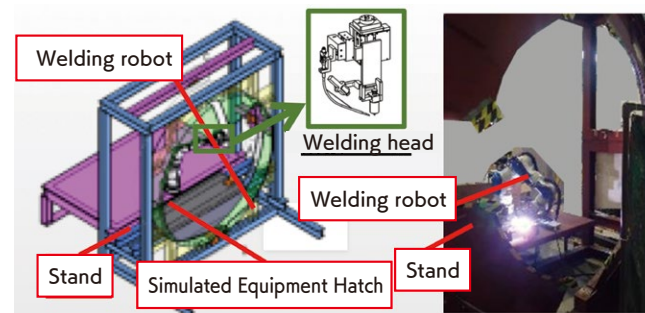
▲ Test welding the access tunnel connection
