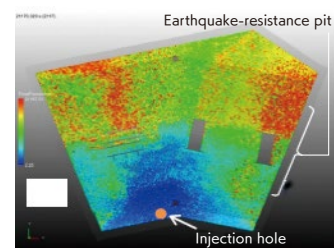
◀ Simulation analysis of filling with reinforcement material (Figure 6)
