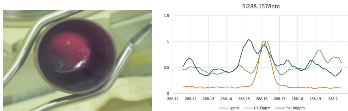
▲ Alkali dissolution testing on simulated fuel debris (Figure 10)
