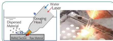
▲ Laser gouging; dispersed material accumulated in specific locations
