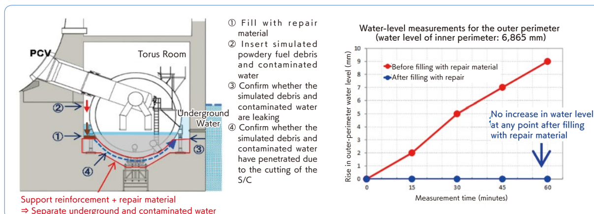
▲ Boundary-effectiveness testing and results (Figure 9)
