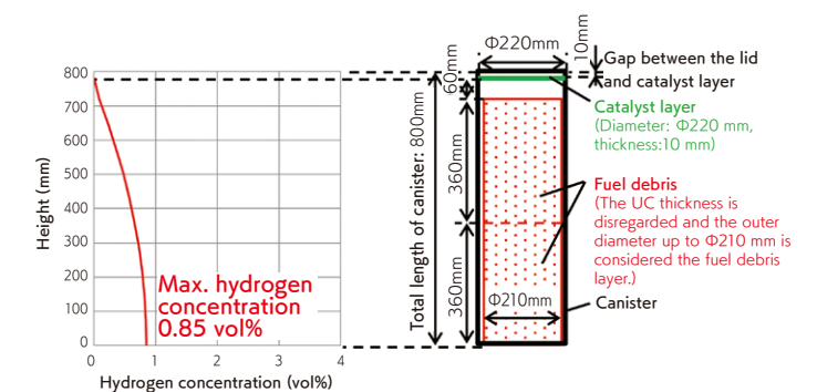
▲ Distribution of hydrogen concentration in canister (figure 8)
