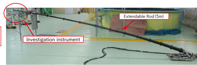
▲ Investigation equipment (with rod extended) (Figure 2-2)
