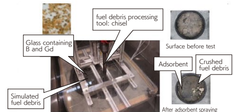
a) Underwater testing with chisel (simulated lower pedestal) b) Surface appearance before and after testing
