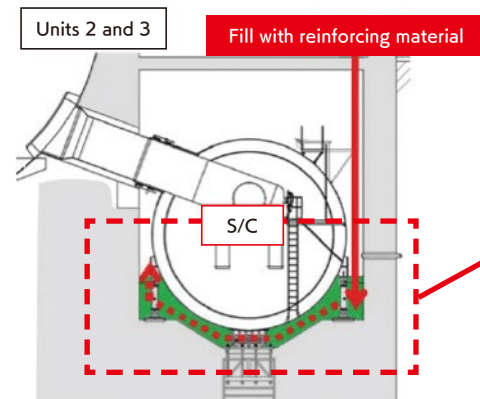
▲ Fill area for reinforcing S/C support columns (Figure 2)
