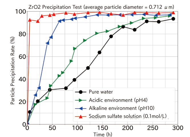
▲ Changes in the ZrO2 particle precipitation rate over time for different dissolved substances (Figure 15)
