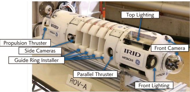
▲ The submersible robot [IRIDOLPHIN-A] (Figure 4-2)
