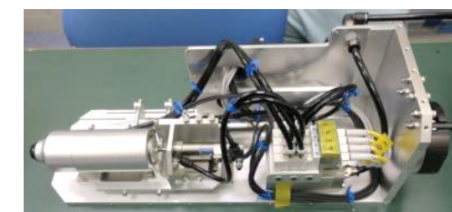
▲ Prototype: Vacuum tube method
