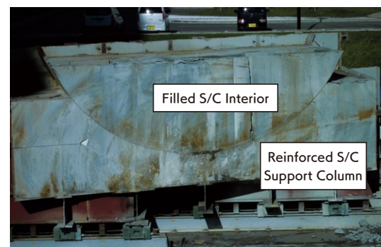
▲ Results of filling test at 1:1 scale (Figure 7)
