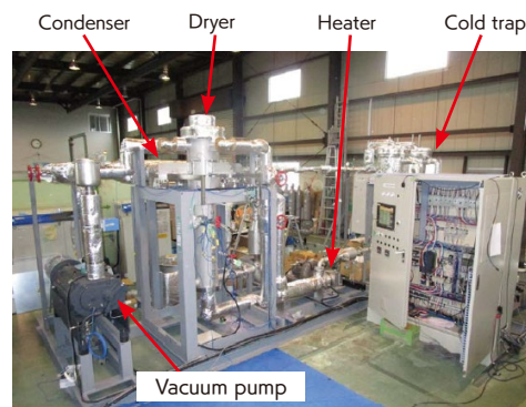
▲ Appearance of full-scale drying test equipment (figure 9) To verify the effects on drying behaviors affected by the drying method and operational conditions, a full-scale drying system was manufactured and verified.
