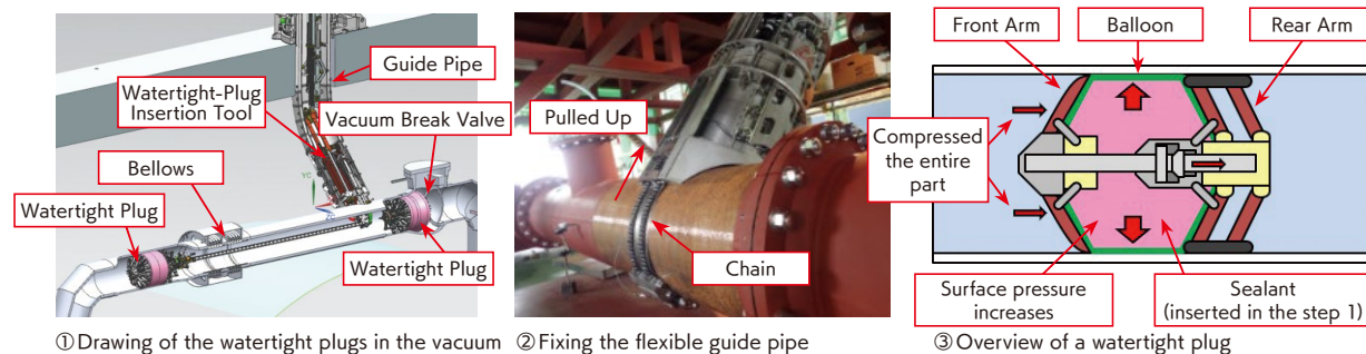
① Drawing of the watertight plugs in the vacuum break line ② Fixing the flexible guide pipe ③ Overview of a watertight plug
