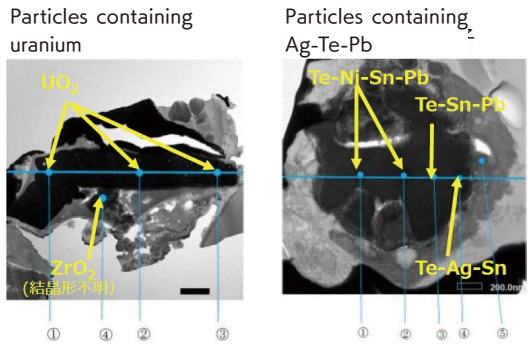
▲ TEM* analysis of fine-powder sample collected from within the SGTS intake pipes of Units 1 and 2 (confirmation of particles containing uranium) (Figure 17) *TEM: transmission electron microscope
