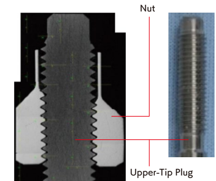
▲ Cross-sectional view of test piece that simulates the upper end of a fuel assembly (left) and results of visual inspection (right) (90 °C, chlorine-ion concentration of 2500 ppm, 1,000 hours of immersion followed by 60 °C, chlorine-ion concentration of 100 ppm, and 7,409 hours of immersion) (Figure 1)
