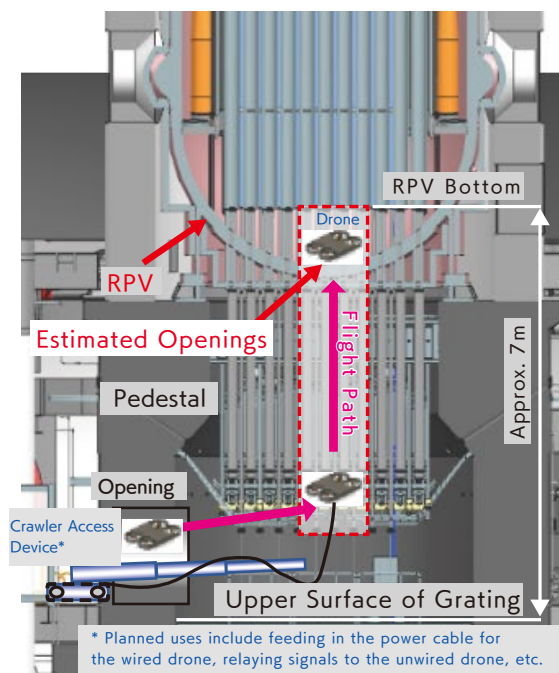
▲ Accessing Unit 1 with a drone (Figure 1)
