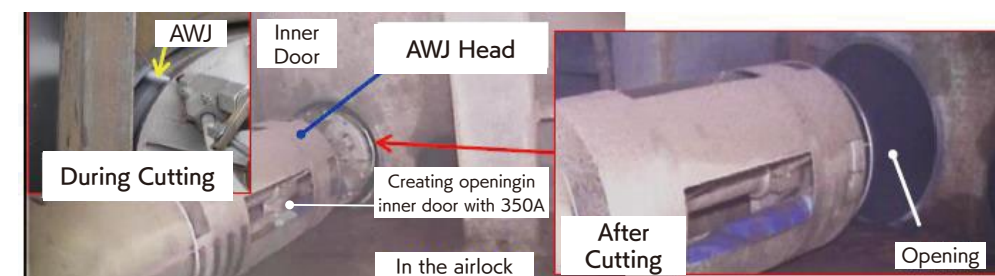
▲ Creating opening in the inner door of the airlock (Figure 3-3)
