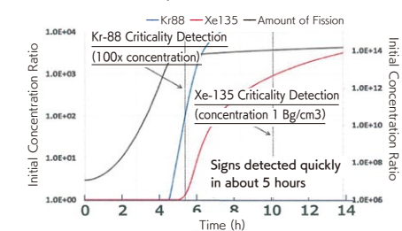
▲ Evaluating criticality detection when a criticality event is suspected (Figure 3)
