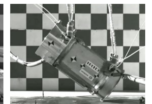
Structural test (dropped at an angle)
