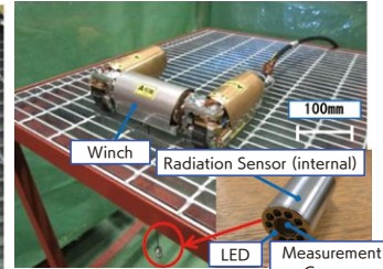
▲ PMORPH2 for investigating the subfloor outside the pedestal (Figure 1-2)
