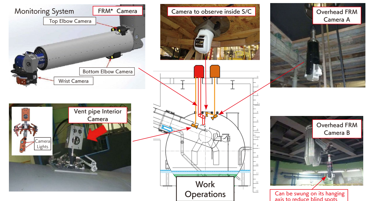
▲ Monitoring cameras installed on remote-operated repair equipment (Photo 4)
