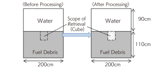
▲ Evaluation system (added reactivity due to the perfect mixture of water and fine fuel debris powder)
