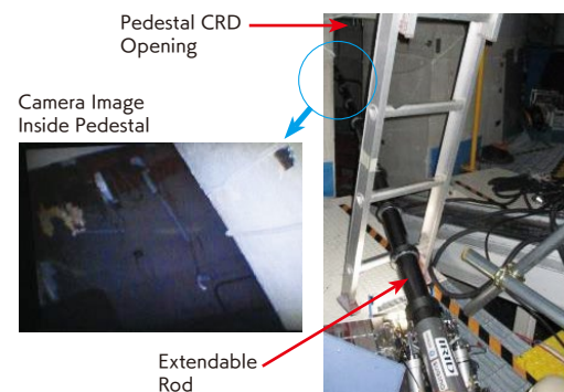
▲ Validation test for continuous operation (Figure 2-3)
