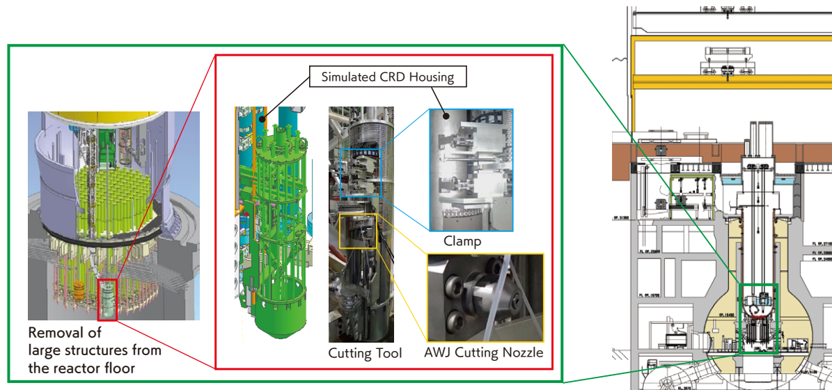
▲ Transport with the cutting method and element testing related to cutting the CRD housing
