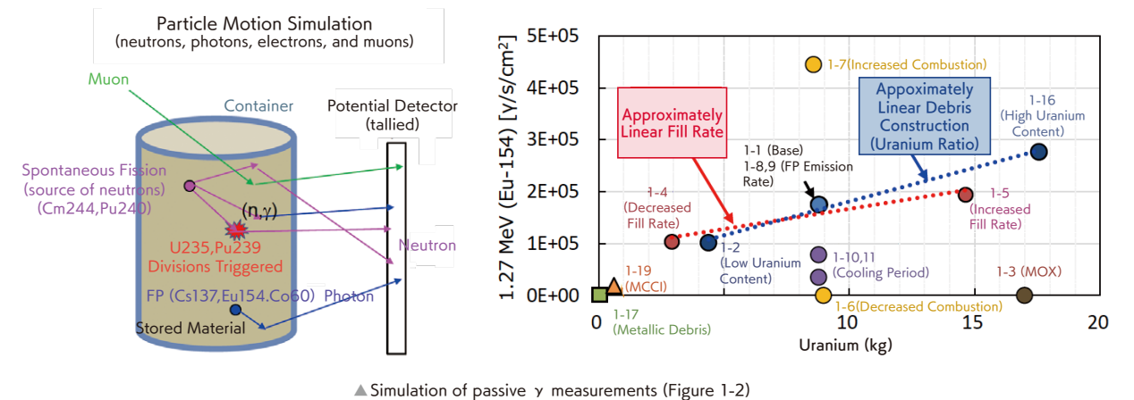
▲ Simulation of passive \gamma measurements (Figure 1-2)
