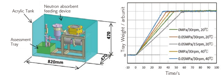
(a) The test setup (b) Changes over time in the amount of adsorbent injected
