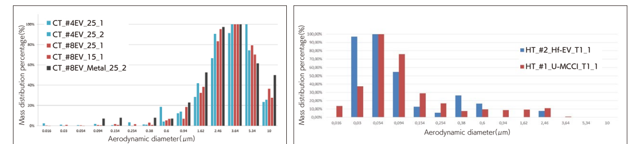
▲ Test results on the generation and behavior of particles using simulated fuel debris that contains uranium from the testing in France (Figure 13)
