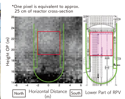
▲ Distribution of matter at the bottom of the RPV (Unit 2) (Figure 5) (measurements taken on July 22, 2016)
