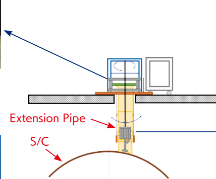
▲ Structure of the S/C water intake (Figure 5)
