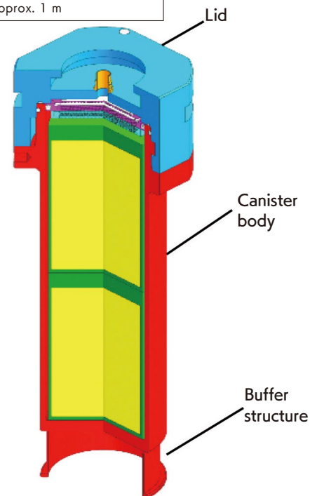
▲ Proposed canister structure (figure 3)
