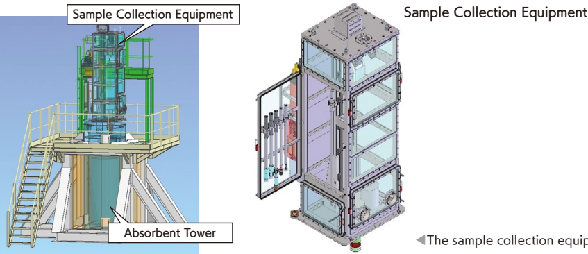
◀ The sample collection equipment for cesium adsorbent towers
