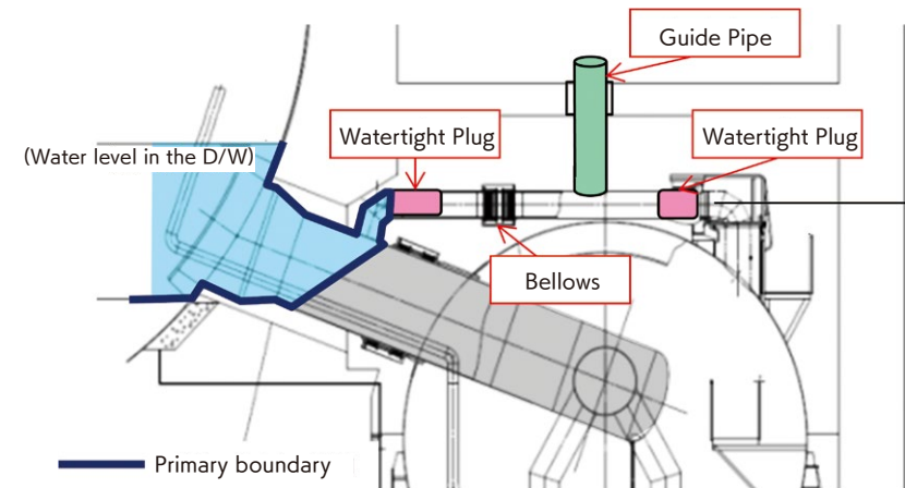
▲ Conceptual image of a method to stop leaks from the vacuum break line (Unit 1)
