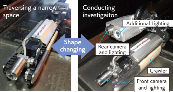
▲ Remote-operated crawler investigation robot (Figure 1-1)
