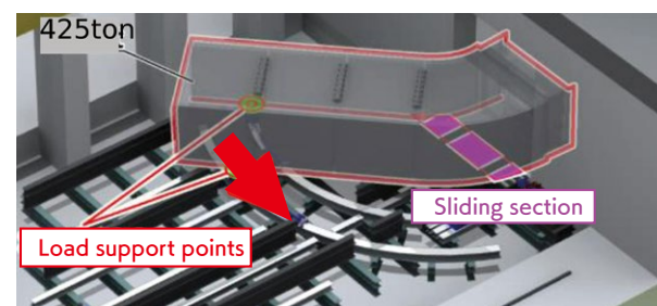
▲ Turning the access tunnel
