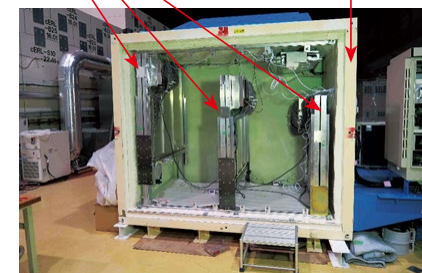
▲ Muon-transmission measuring device (Photo 1) (Dimensions: approx. 2.5m×2.0m×2.1m [height])
