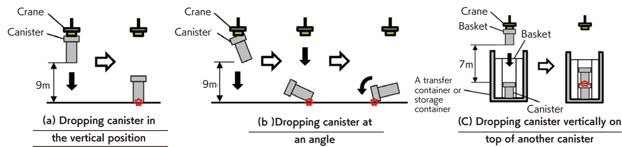
▲ Conceptual images of drop events (figure 2)
