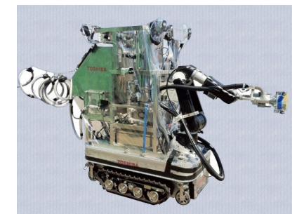
▲ Dry-ice blast decontamination equipment (Figure 3)
