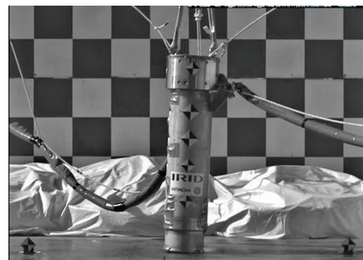
▲ Structural test (dropped vertically) (figure 4)
