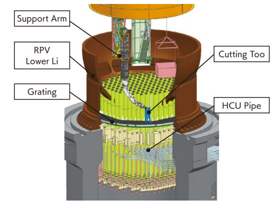
▲ Removing obstacles from the bottom of the reactor
