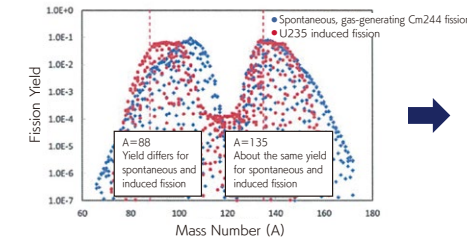
▲ Yields for spontaneous and induced fission
