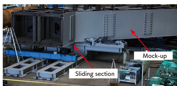
▲ Full-scaled weight simulated access tunnel
