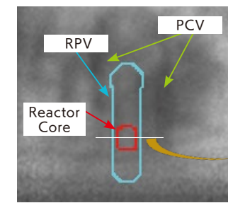
▲ Distribution of muon-transmission rate (Figure 3) (Reactor 1; measured February–May 2015)
