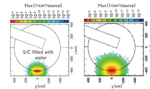
Calculation results for Eu-154 Calculation results for Cm-244 ▲ Distribution of fuel-originating radiation in the vicinity of Unit 1's S/C (Figure 2)
