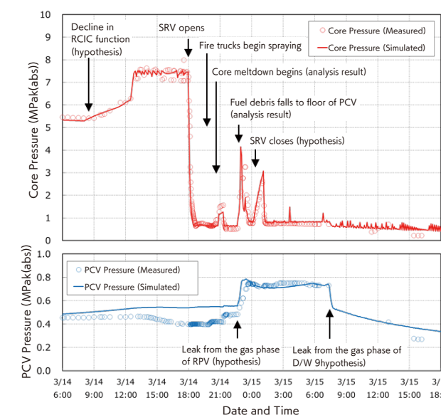
▲ Using MAAP codes to reproduce the events of the Unit 2 accident progression
