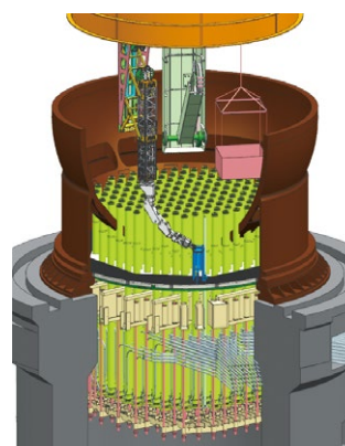
Removing obstacles from the bottom of the reactor
