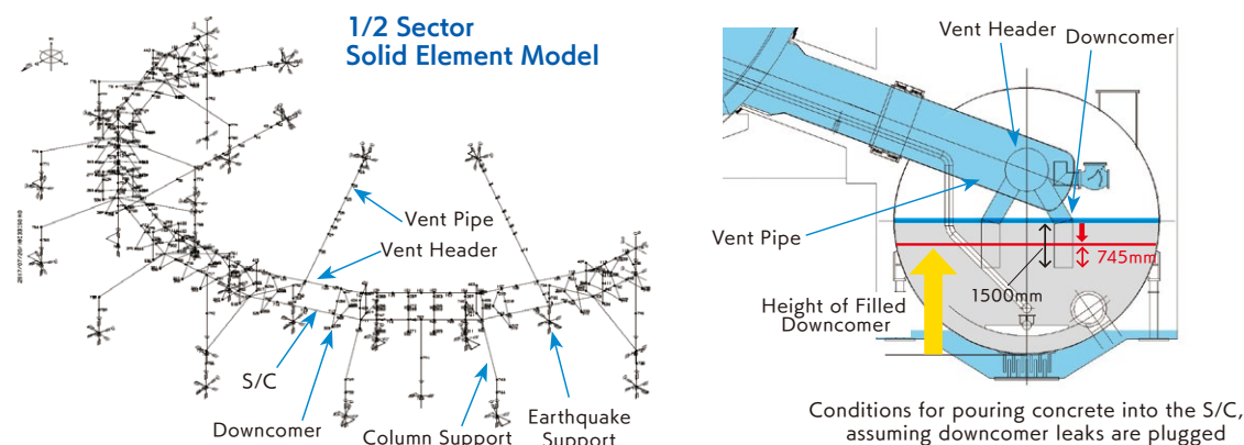
▲ Time-history earthquake response model (Units 2 and 3) and conditions for linkage analysis of vent pipe and S/C system (Figure 6)
