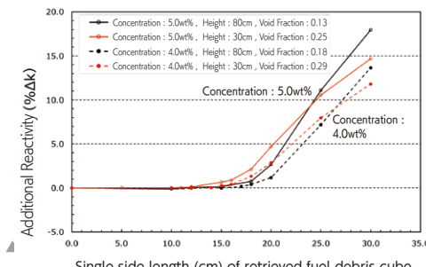
▲ Relationship between additional reactivity and the amount of debris retrieved per shift (Figure 1)
