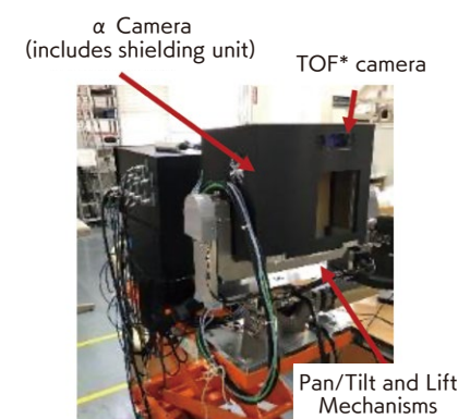
▲ The measurement device (Figure 7)
