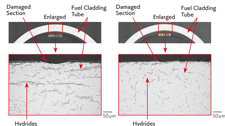
▲ Results of hydride precipitation test (300 °C, cooling rate of 0.3 °C/h, circumferential stress of 70 MPa, damaged) (Figure 4)
