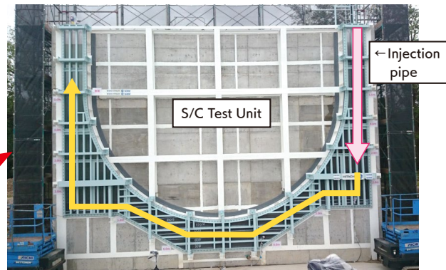
▲ S/C support column validation test (1:1 scale; simulates Units 2 and 3) (Figure 3)
