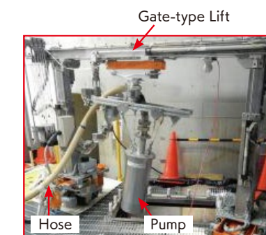
▲ Inserting the pump into the D/W basement floor (Figure 4)
