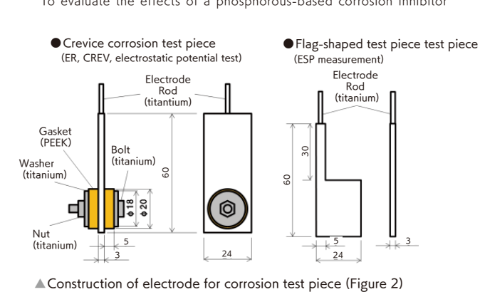
▲ Construction of electrode for corrosion test piece (Figure 2)
