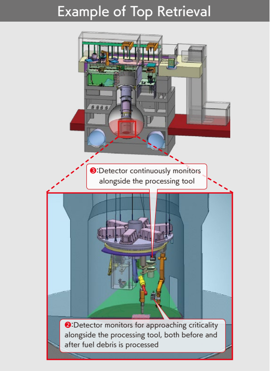
▲ Monitoring for approaching criticality when retrieving PCV fuel debris from the top
