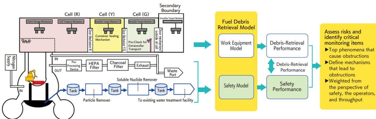
▲ Protocol for identifying critical monitoring items for the PCV interior (Figure 2)
