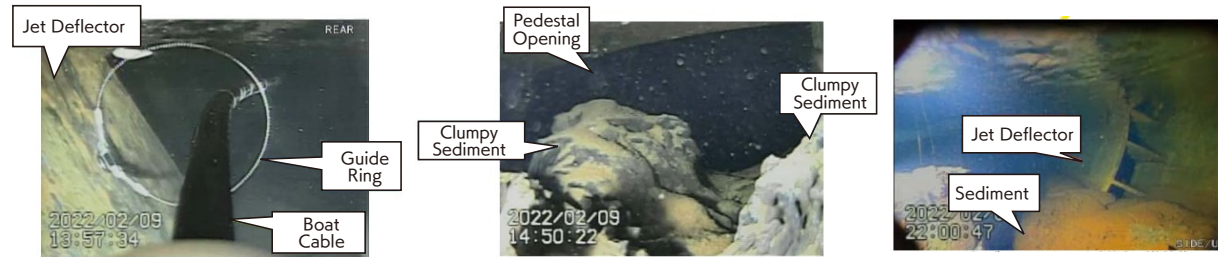
▲ Images of submersible robot [IRIDOLPHIN-A] in action with installed guide rings (Figure 4-4)
