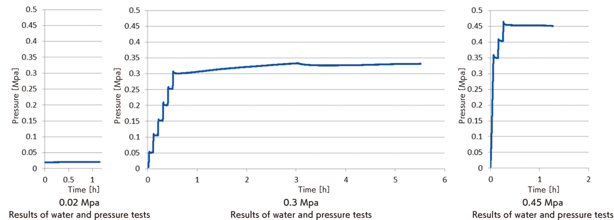
▲ Results of pressure test (Figure 15)
