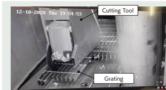
Testing the removal of simulated grating
