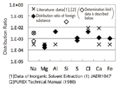
(a) Distribution of foreign substance during the presence of simulated FP FP = fission product
