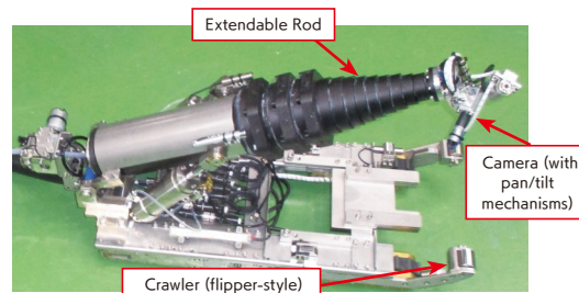
▲ Survey equipment (with rod collapsed) (Figure 2-1)
